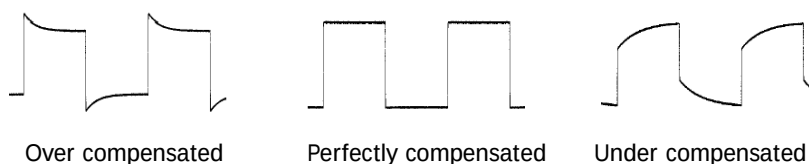
Figure 9 Probe Compensation
