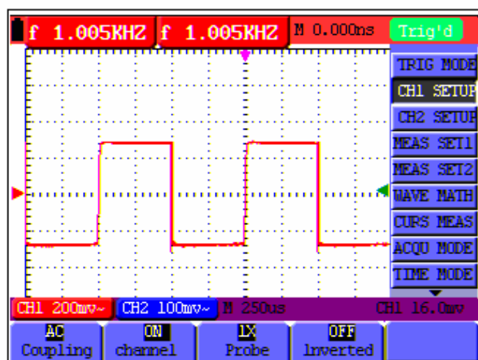
figure 35: AC Coupling
