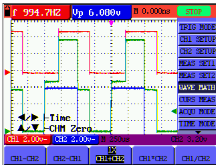
figure 19: Waveform Mathematics
