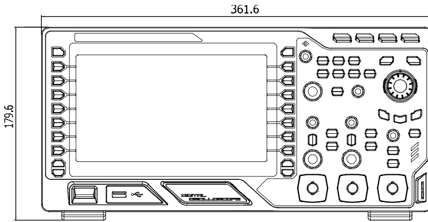
Figure 1 Front View
