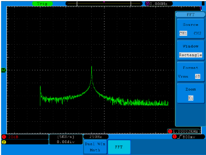
Fig.5-8. Rectangle window
