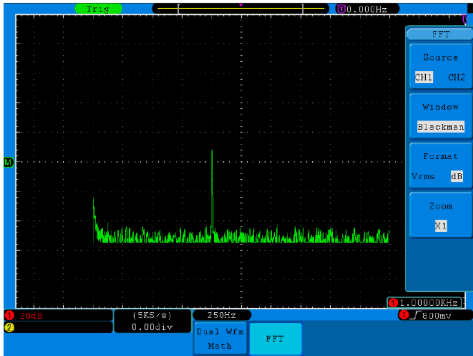
Fig.5-11. Blackman window
