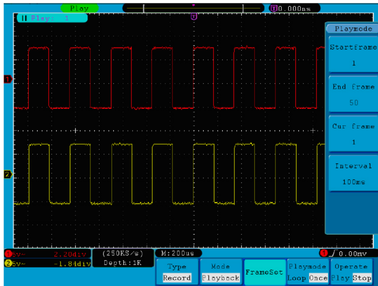
Fig.5-37 Wave Playback
