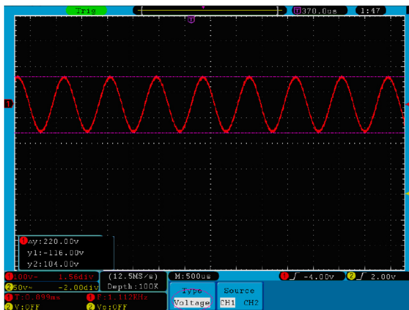
Fig.5-58 Waveform of Voltage Cursor Measurement
