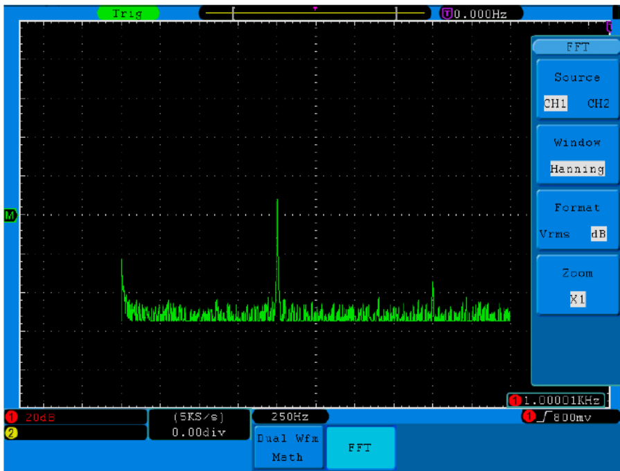
Fig.5-10 Hanning window
