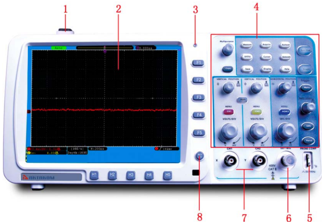
Fig. 4-1 Front panel
