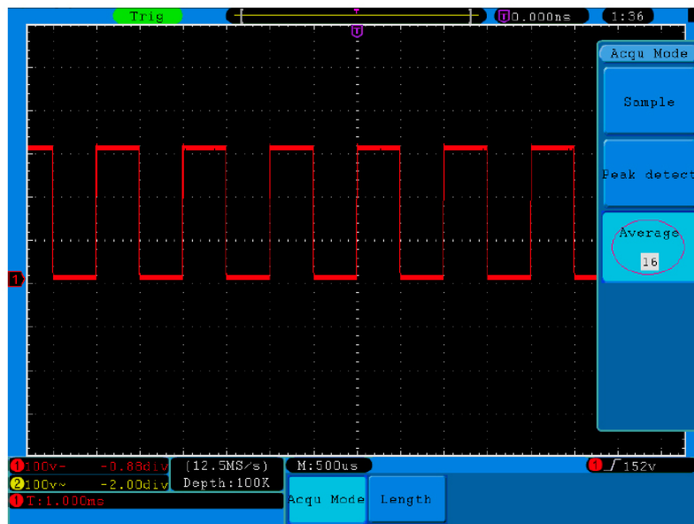
Fig.6-5 Reduce Noise level by using Average function
