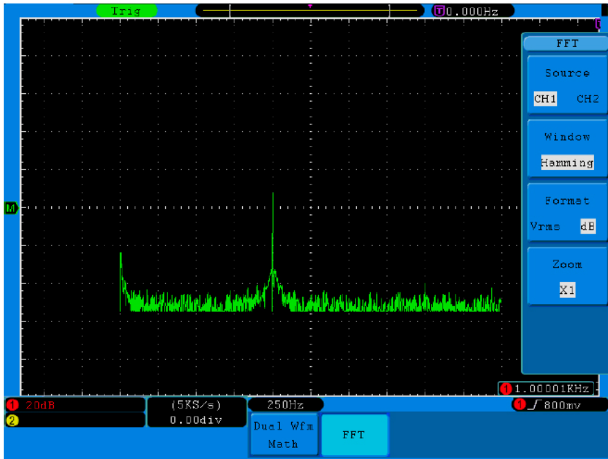
Fig.5-9 Hamming window
