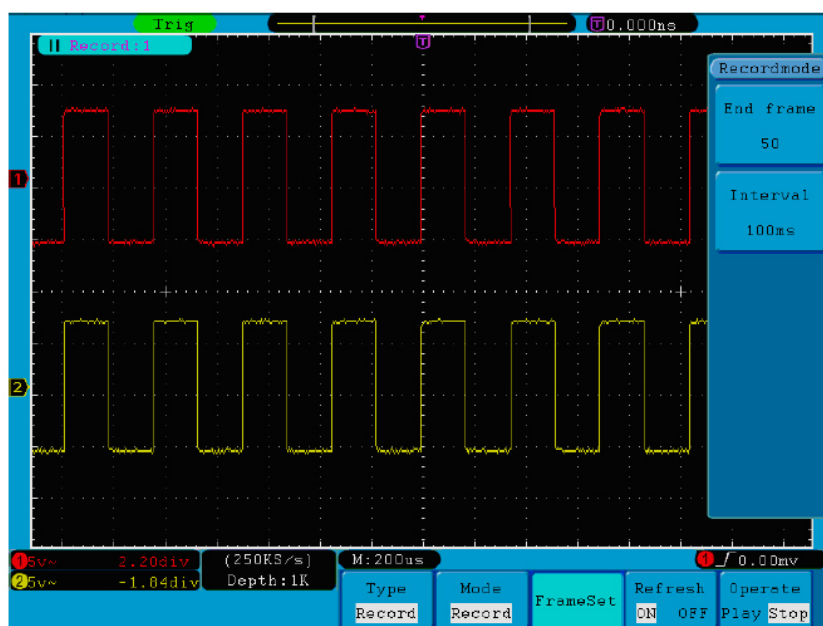
Fig.5-36 Wave Record
