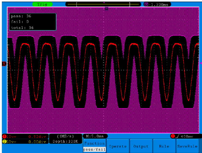
Fig.5-44 Pass/Fail test
