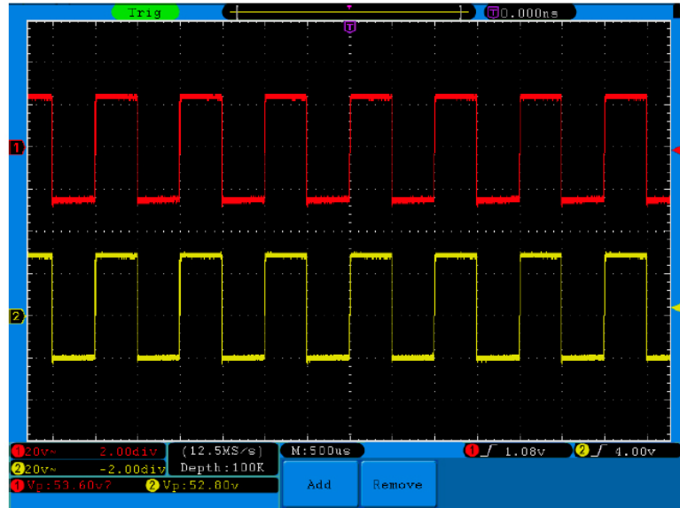
Fig.6-2 Waveform of Gain Measurement
