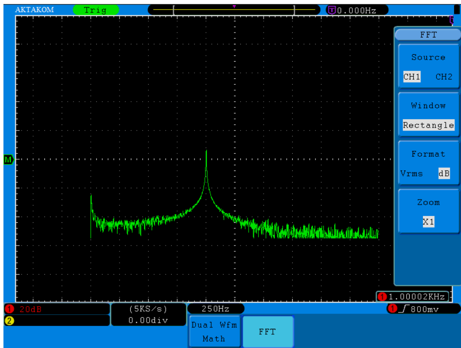
Fig.5-10. Rectangle window
