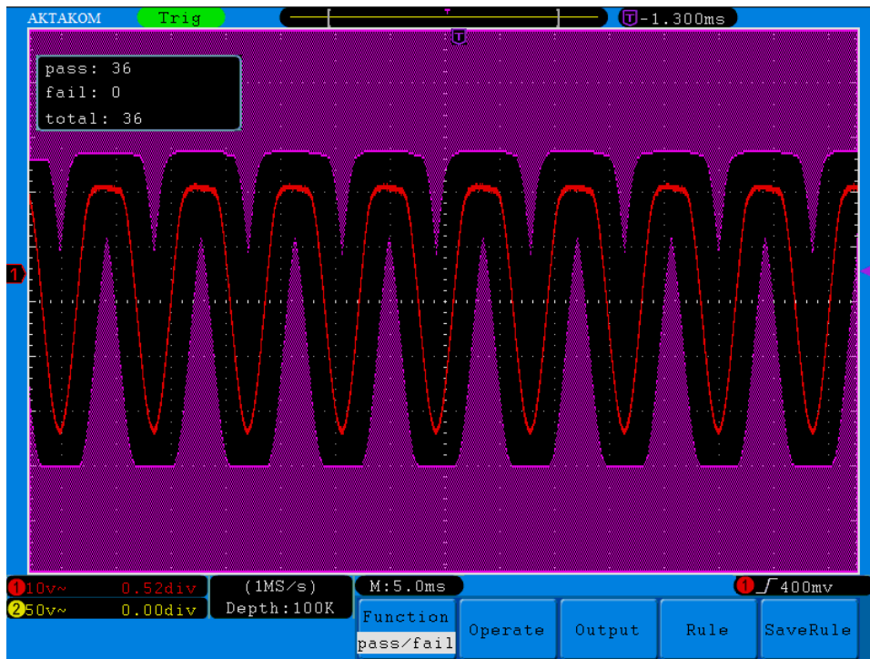
Fig.5-44 Pass/Fail test
