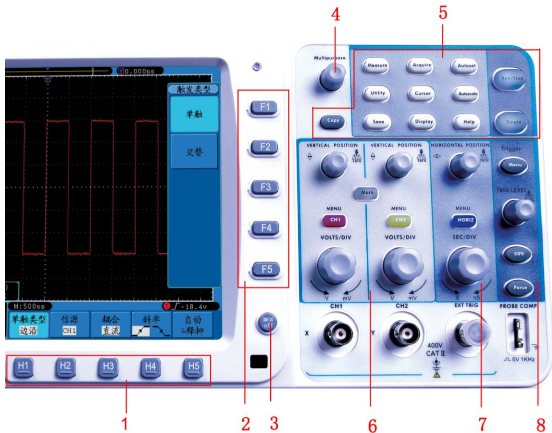
Fig. 4-5 Keys Overview
