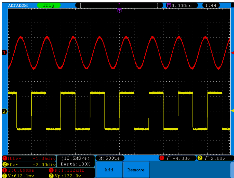
Fig.5-47 automatic measurement
