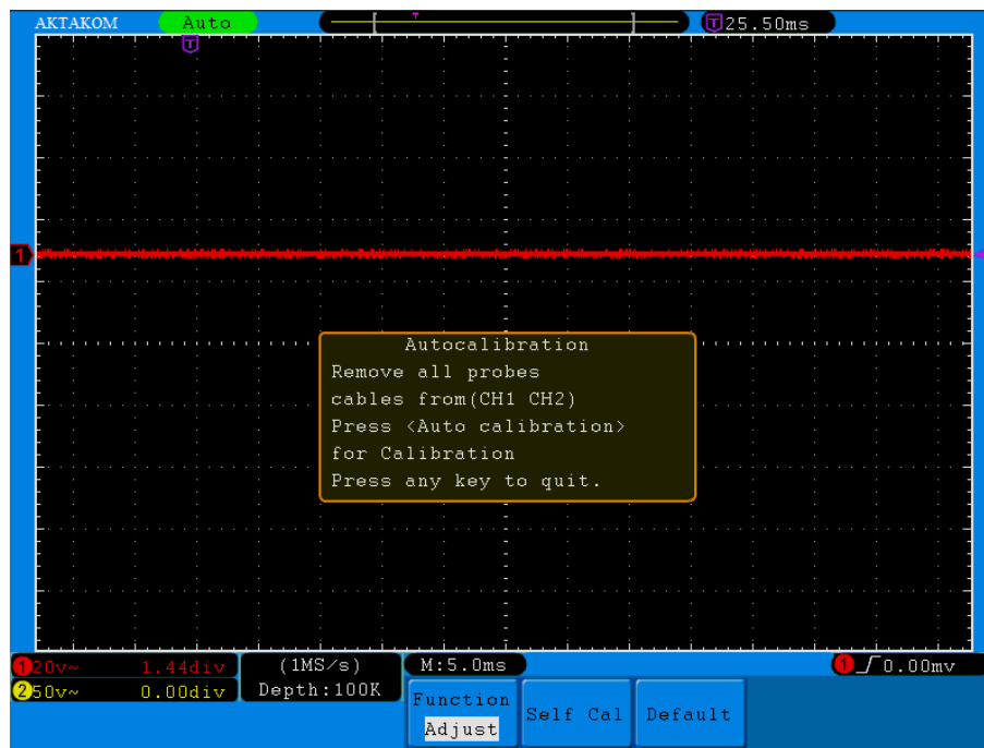
Fig.5-42 Self-Calibration
