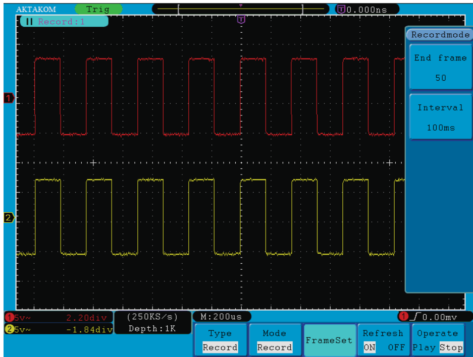
Fig.5-36 Wave Record
