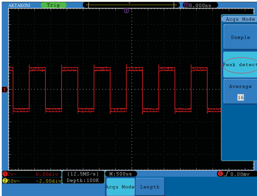
Fig.5-26 Peak Detect mode, under which the burrs on the falling edge of the square wave, can be detected and the noise is heavy.
