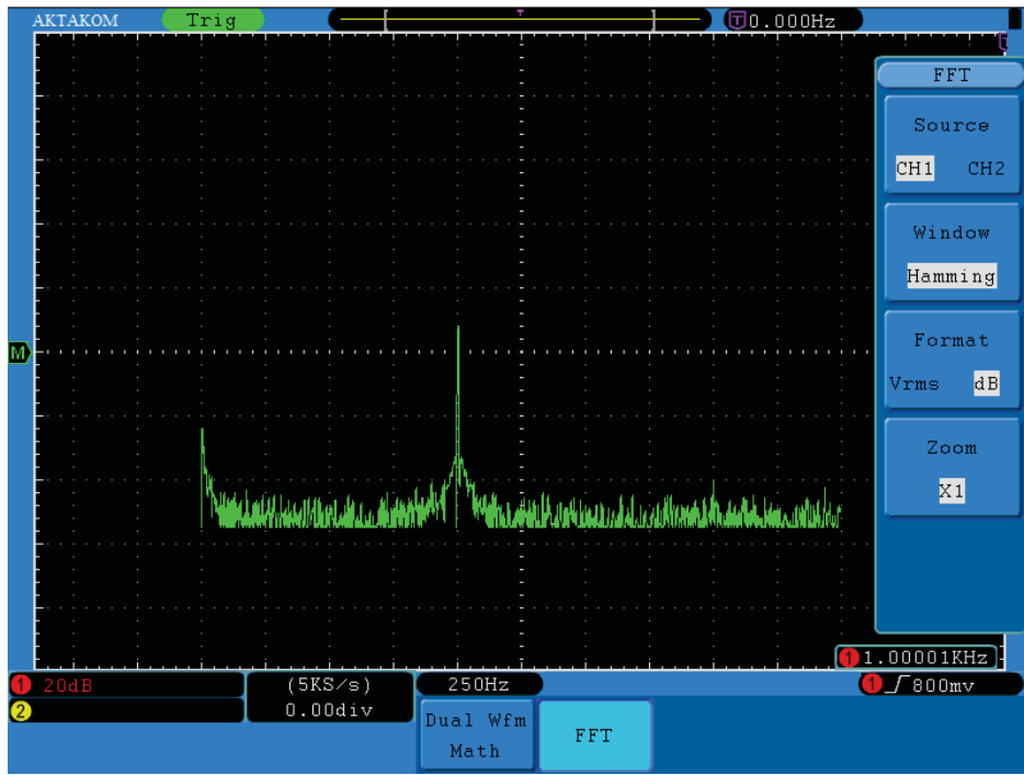
Fig.5-9 Hamming window
