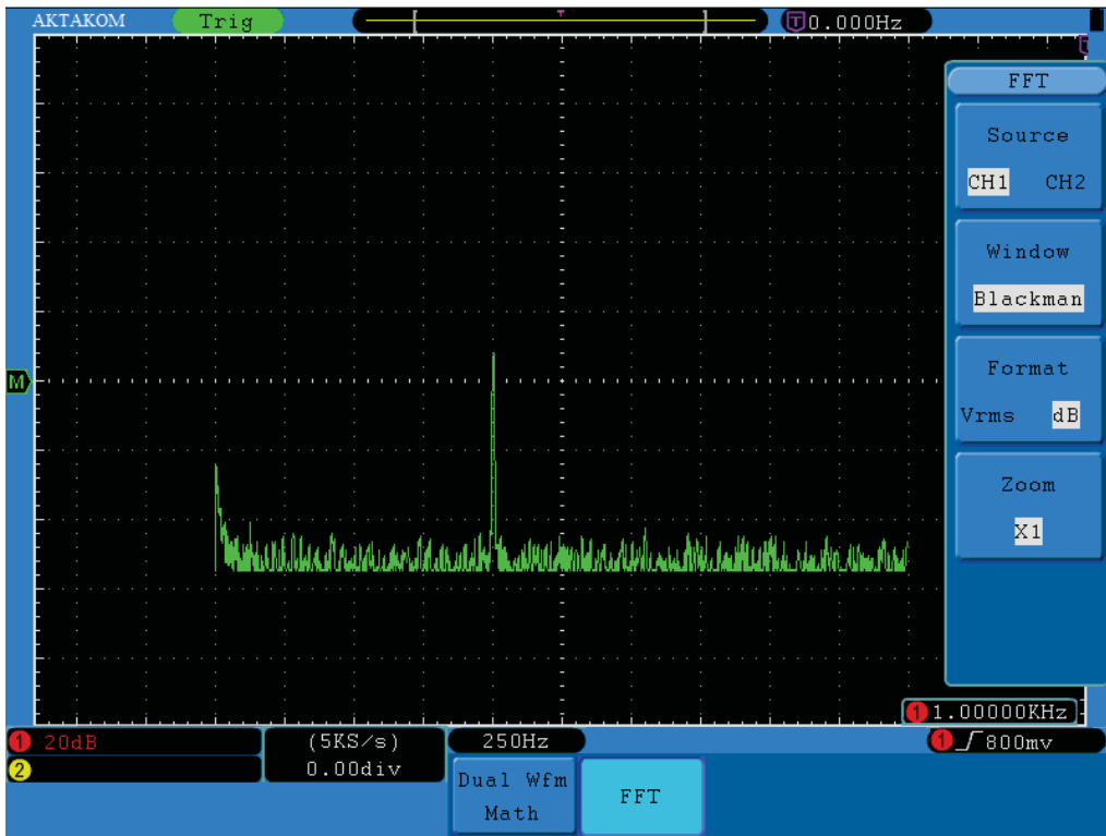
Fig.5-8. Blackman window
