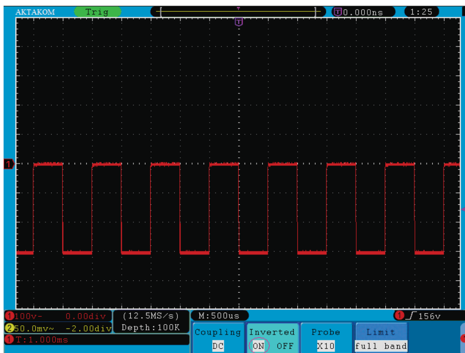
Fig. 5-5 Waveform Inverted
