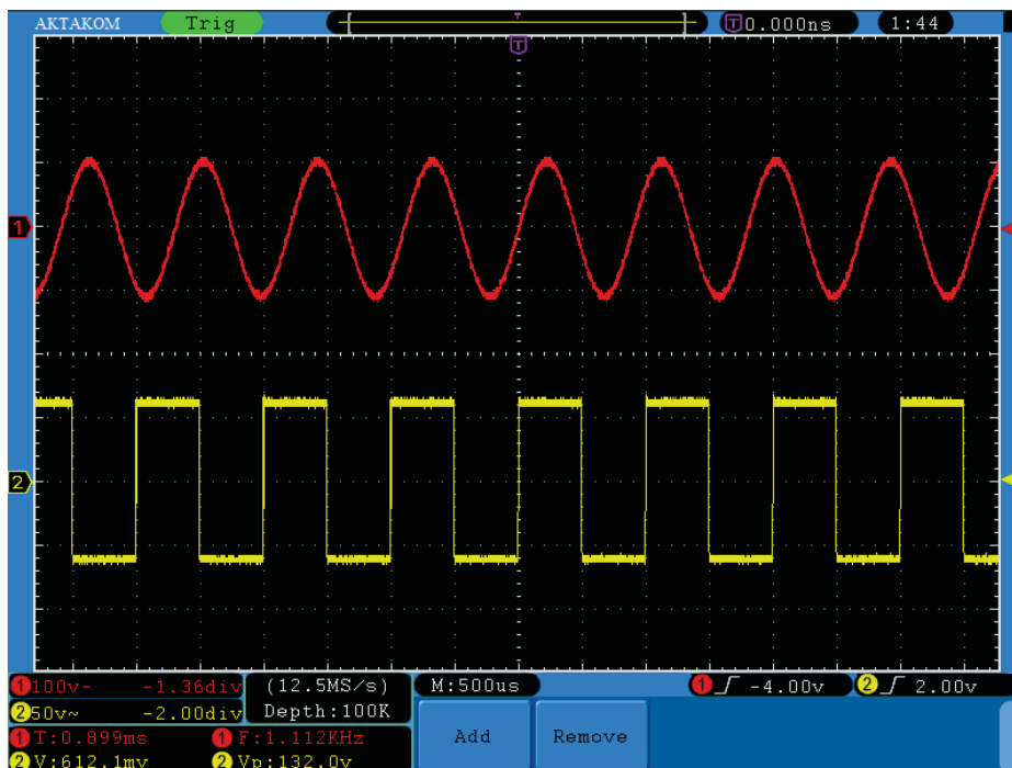
Fig.5-47 automatic measurement
