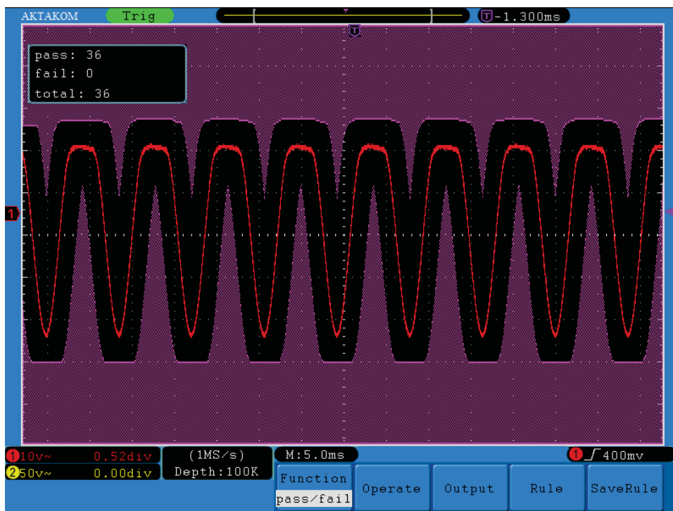
Fig.5-44 Pass/Fail test
